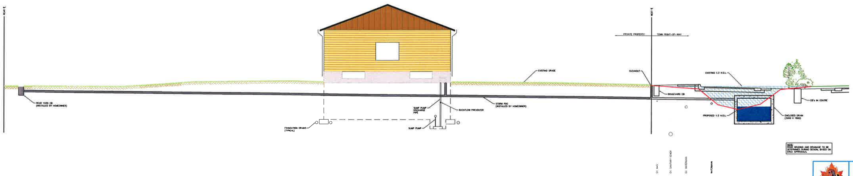
MANNING ROAD TYPICAL UTILITY CROSS SECTION SECTION A-A
