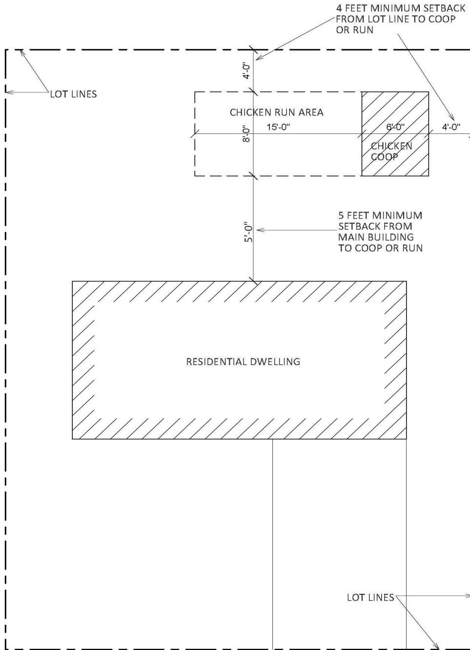
TYPICAL SITE PLAN
