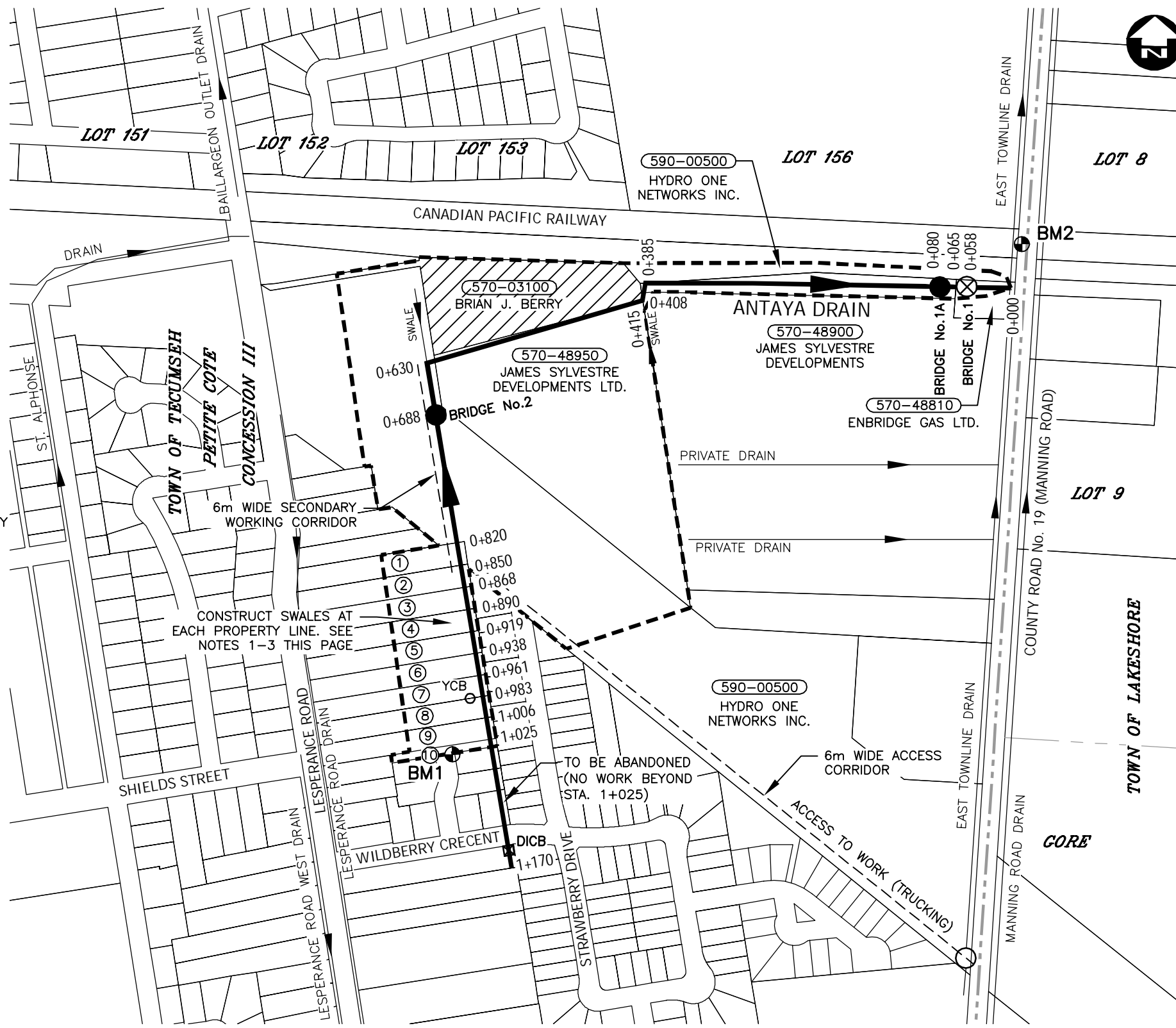
OVERALL PLAN SCALE=1:5,000
