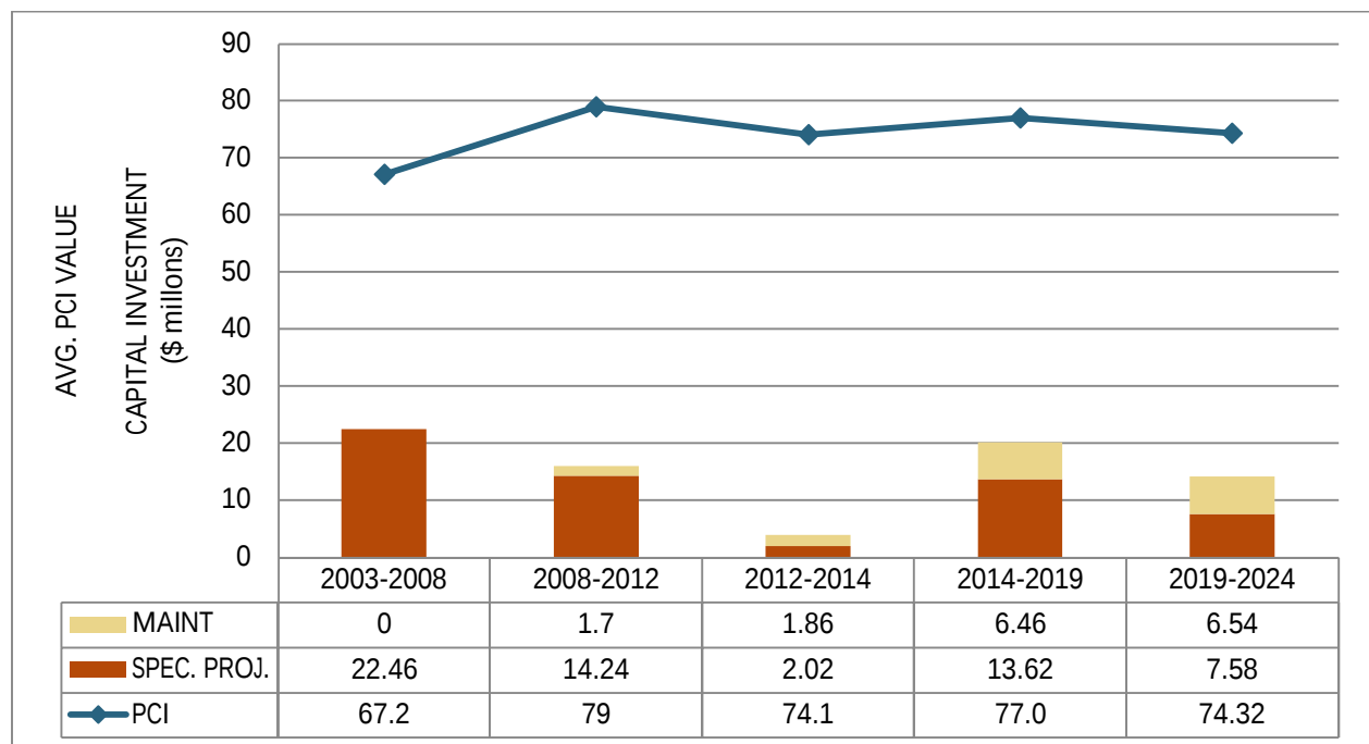
Figure 5-1: Effects of Road Expenditure on PCI
