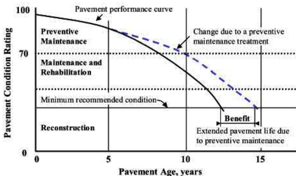
Figure 3-4: Effects of Preventative Maintenance (National Research Council, 2003)
