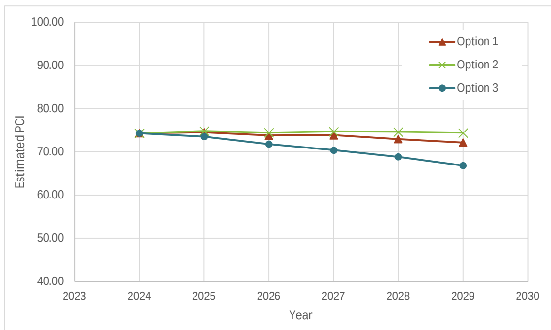
Figure 3-6: Estimated Annual Effects of Maintenance Programs on PCI Values
