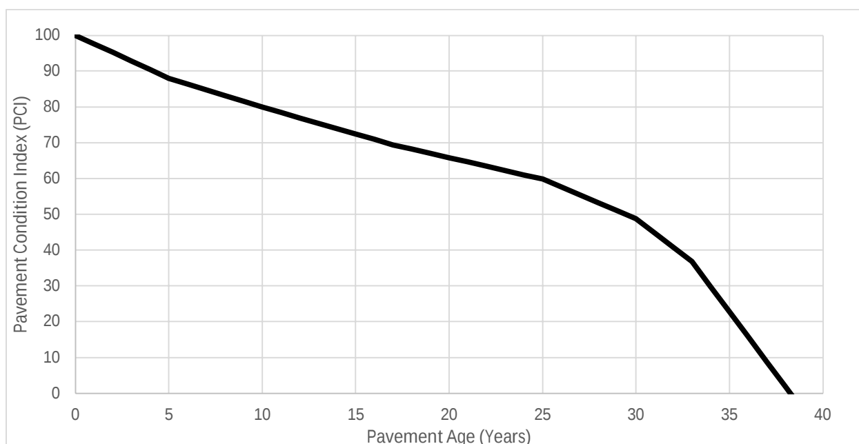
Figure 3-5: Town of Tecumseh Pavement Degradation Curve
