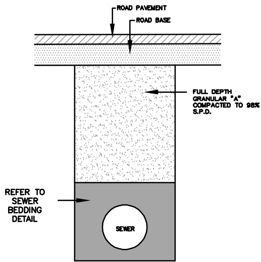
BACKFILL DETAIL WITHIN ROAD AREAS NOT TO SCALE
