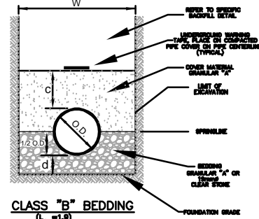
BEDDING FOR RIGID AND FLEXIBLE PIPE SEWERS
