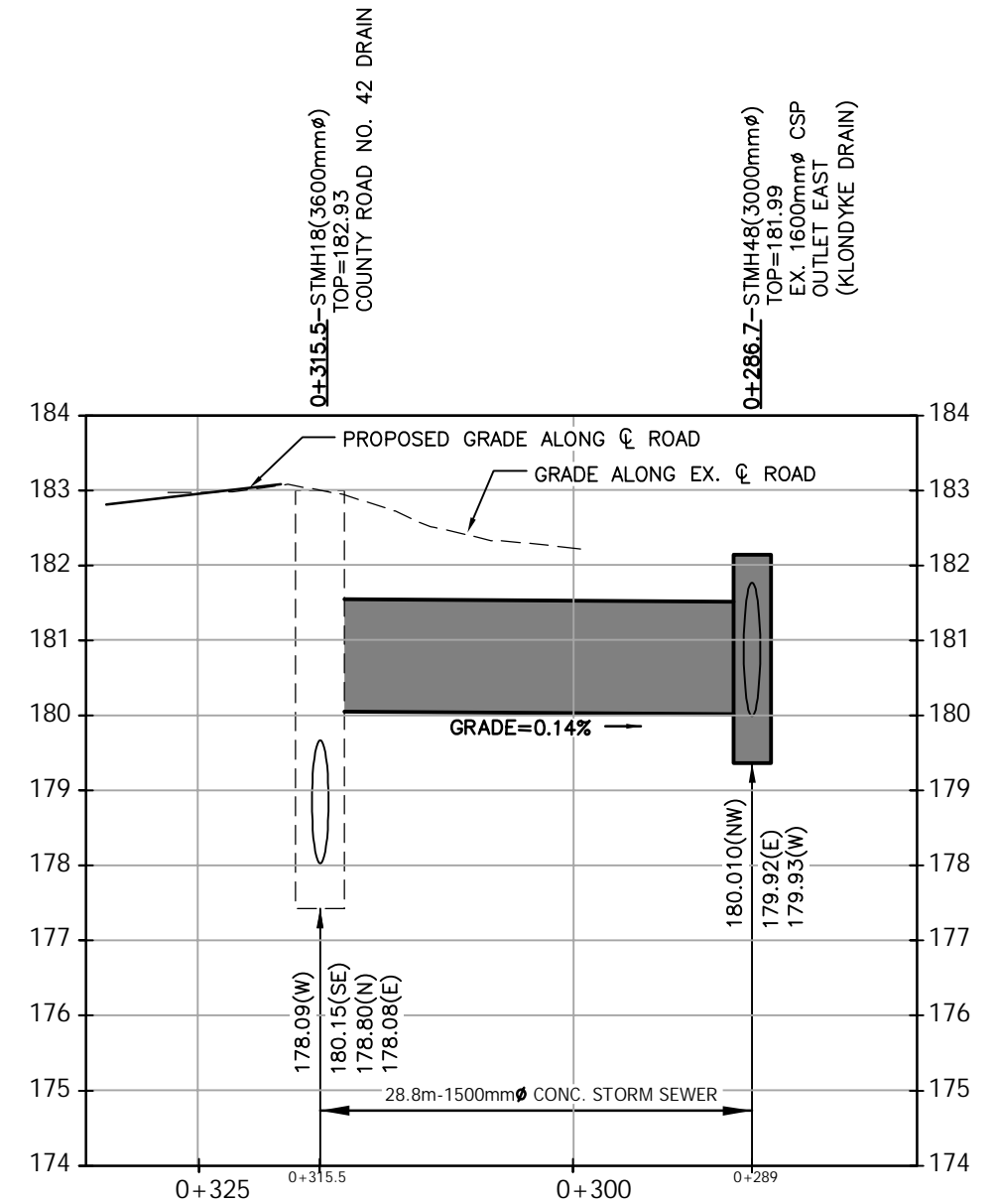
PROFILE (KLONDYKE OVERFLOW DRAIN) SCALE-HORIZ.=1:500 VERT.=1:10
