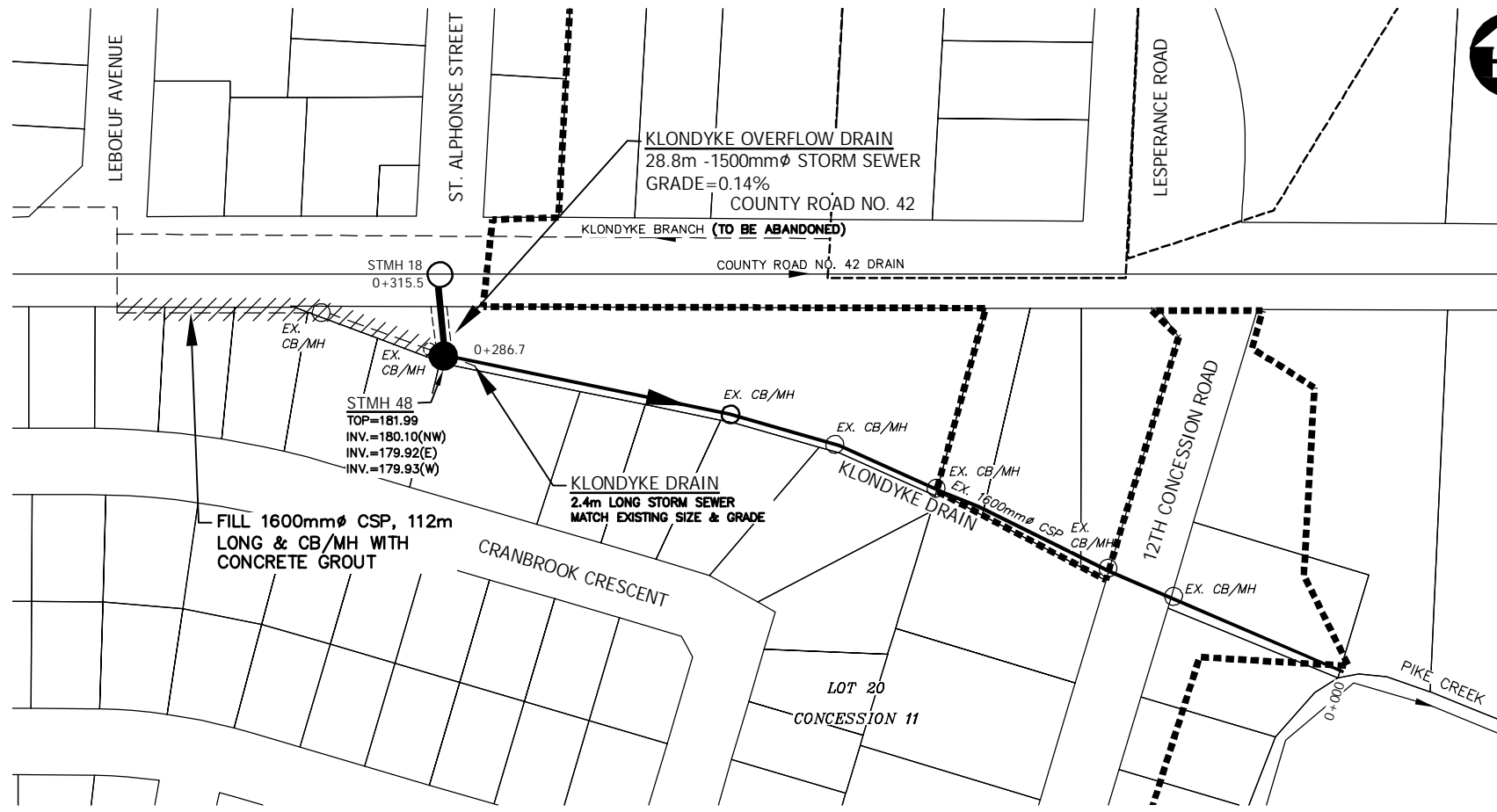
DETAIL SCALE=1:2,000
